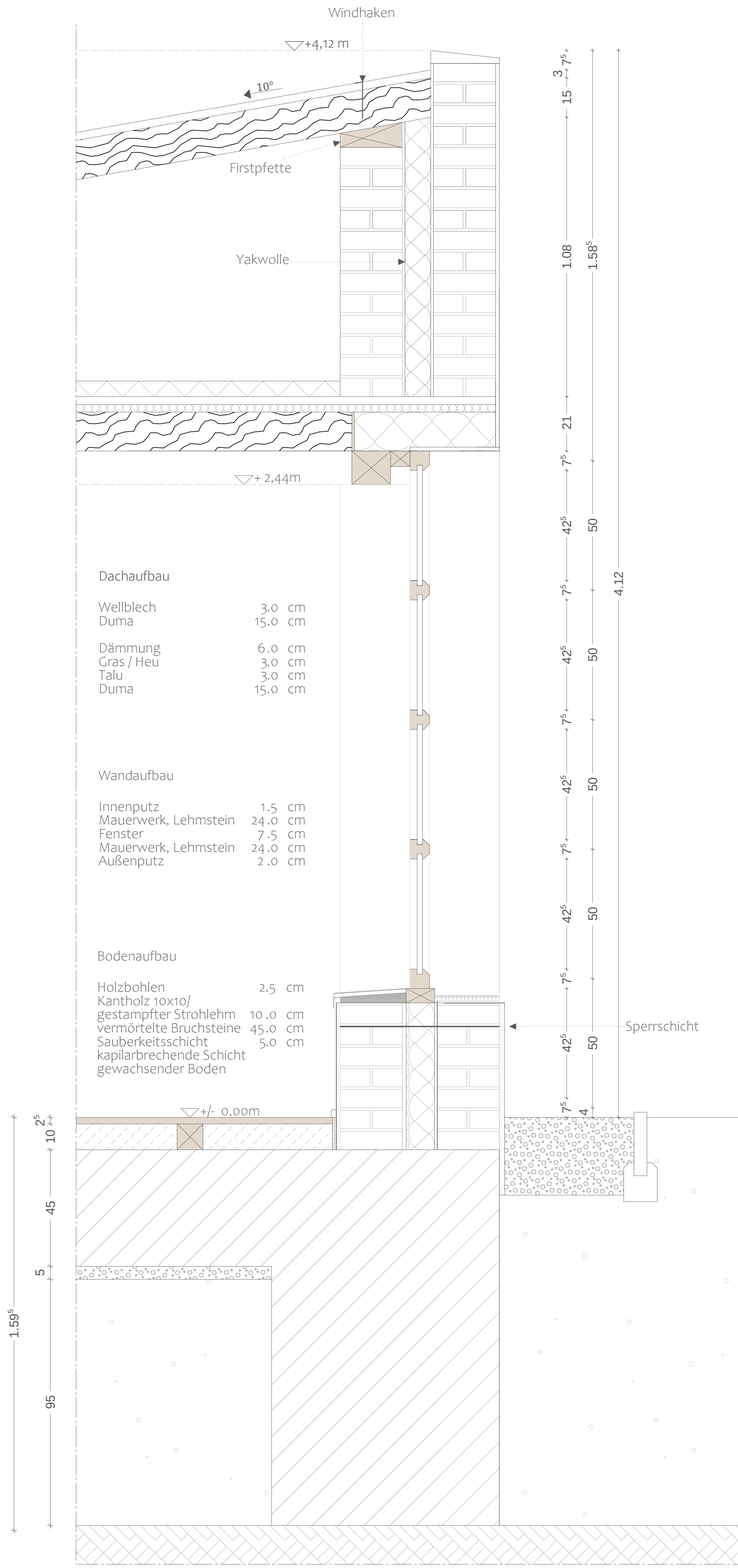
| DETAIL C. Trombewand 1:10
