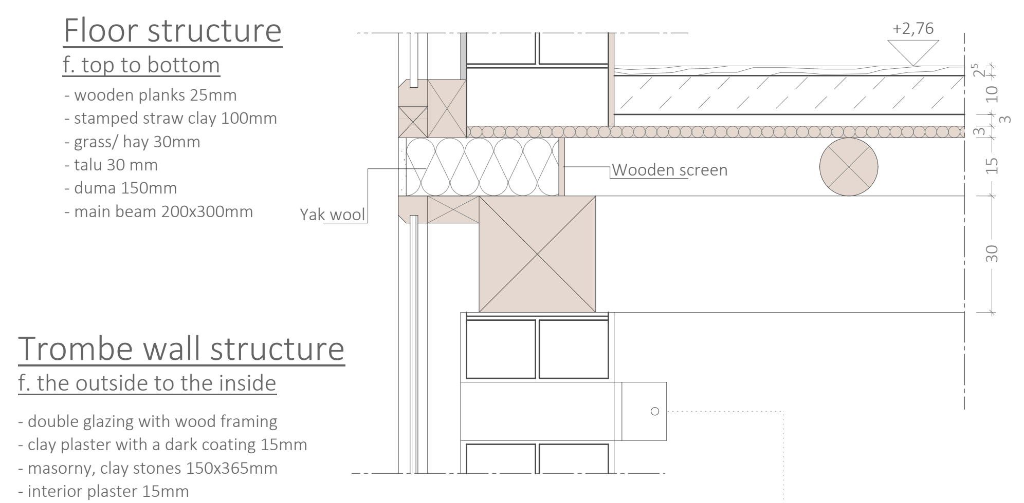
CONSTRUCTION DETAIL D M 1:10
