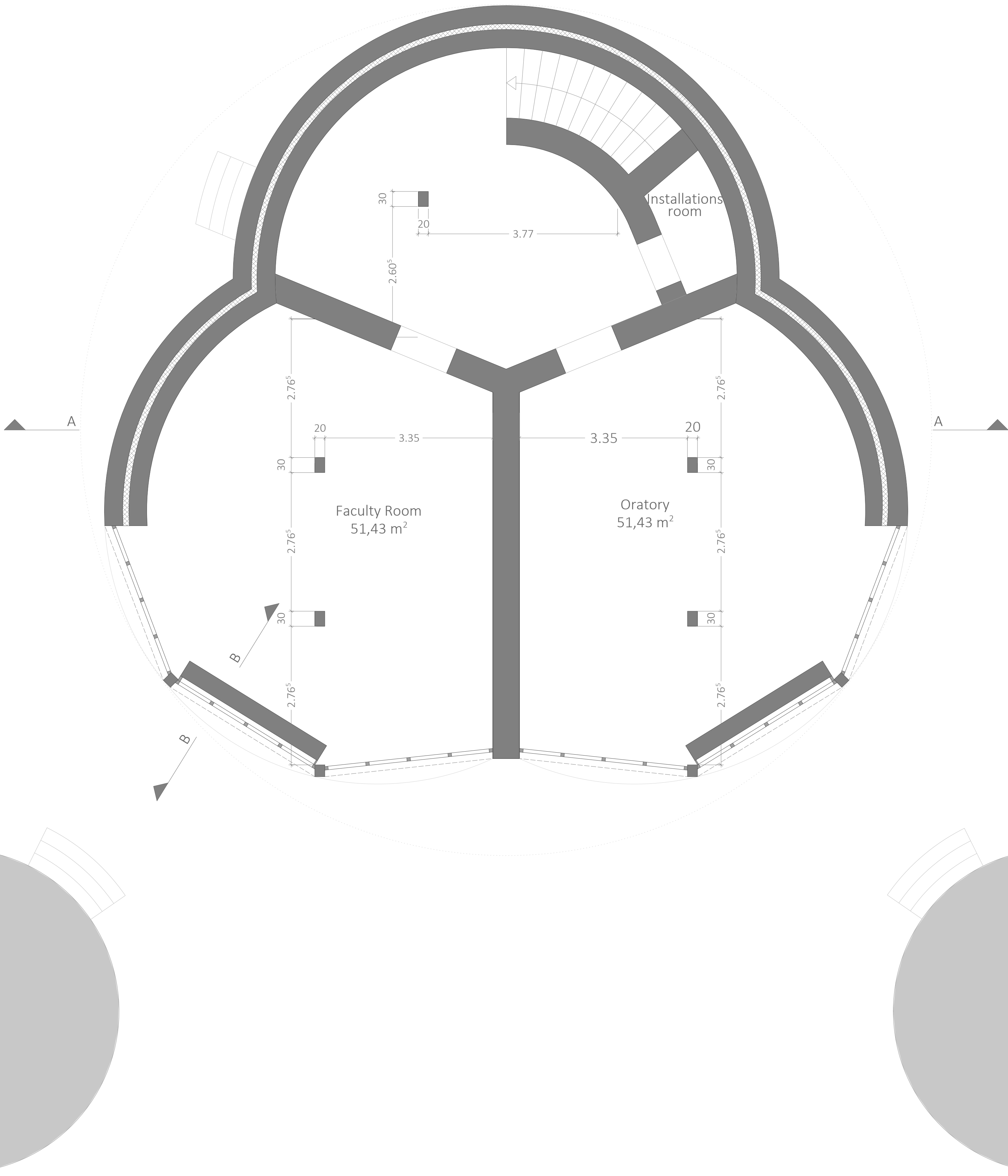
FIRST FLOOR PLAN M 1:50
