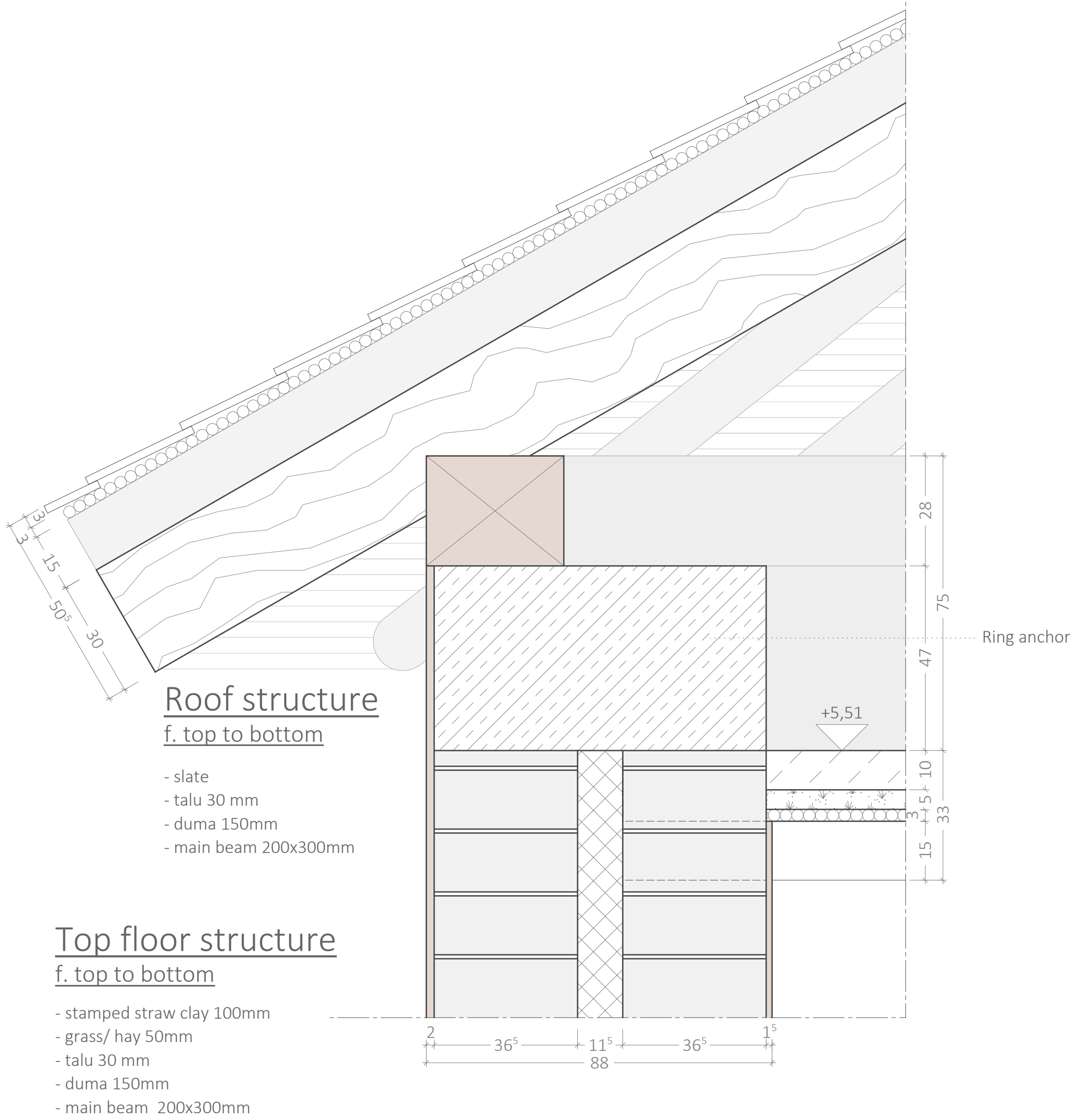
CONSTRUCTION DETAIL B M 1:10
