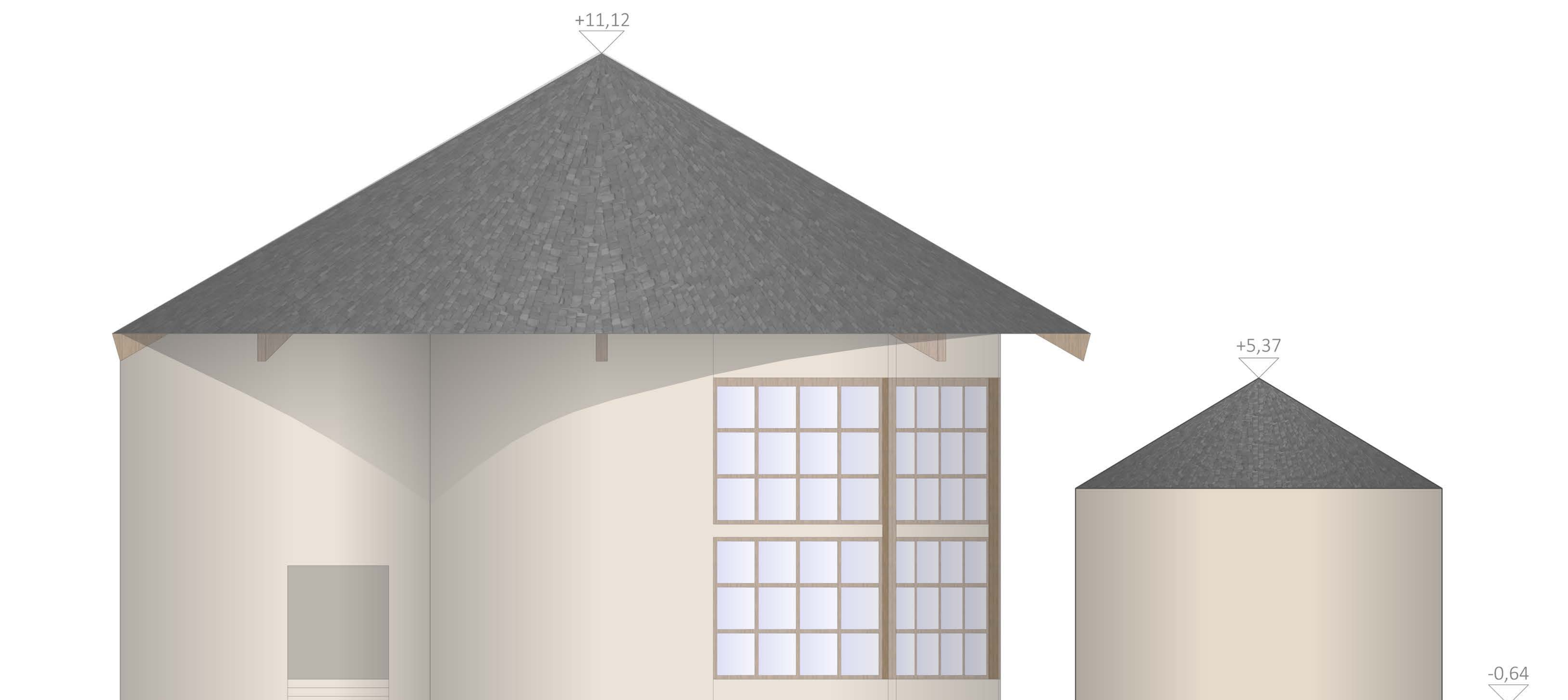
EAST ELEVATION M 1:50
