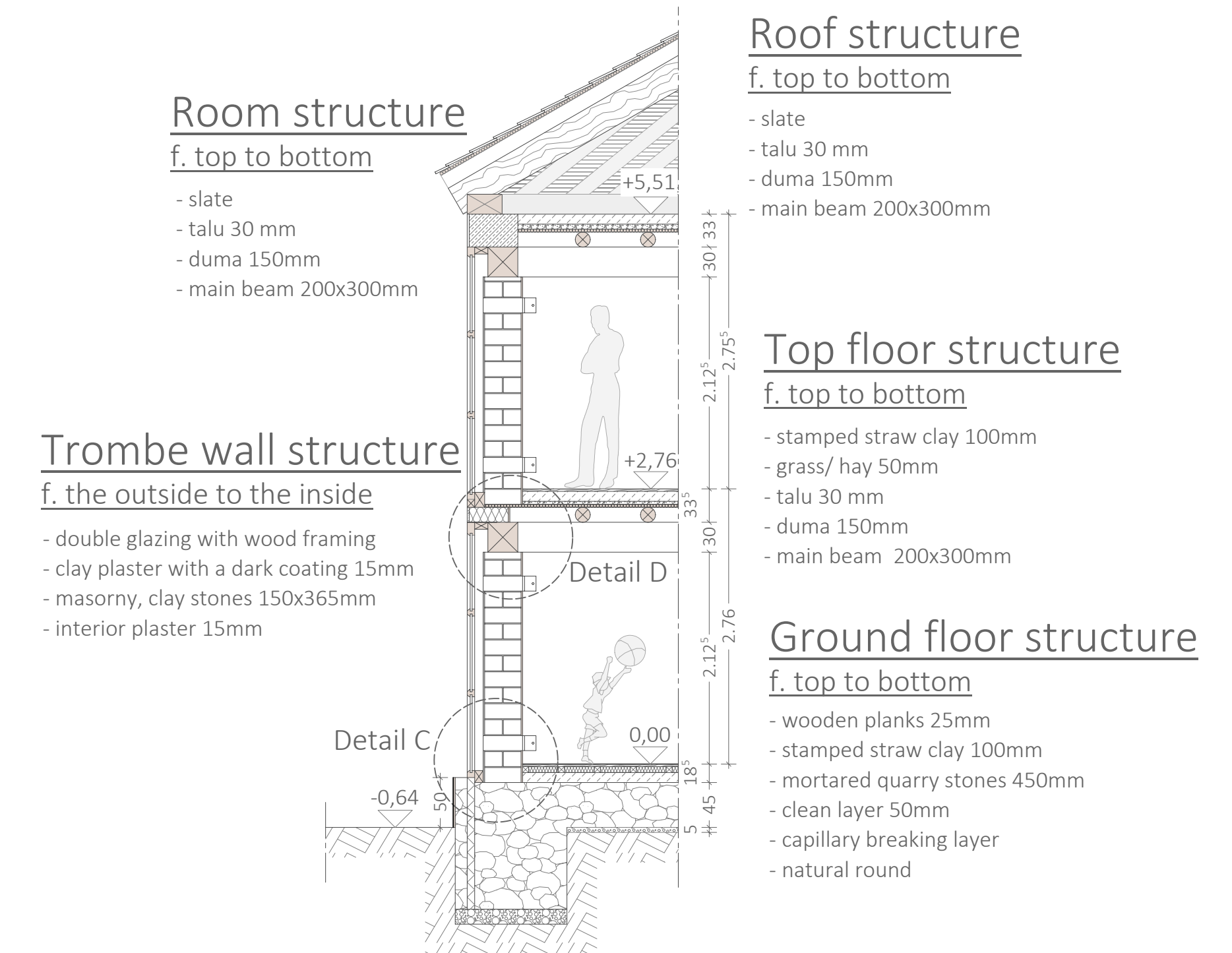
SECTION B-B M 1:50
