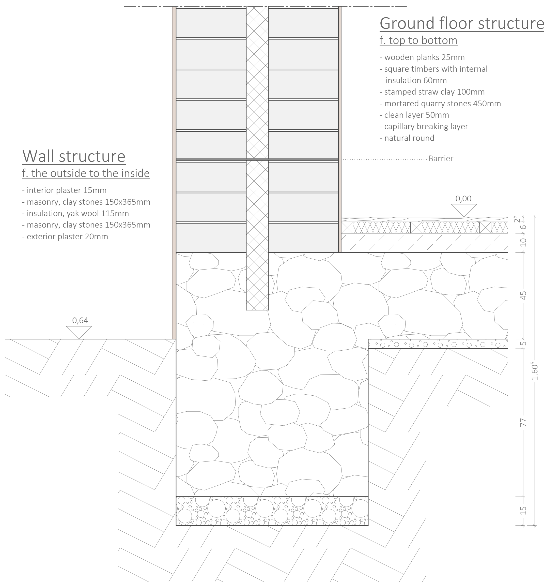
CONSTRUCTION DETAIL A M 1:10
