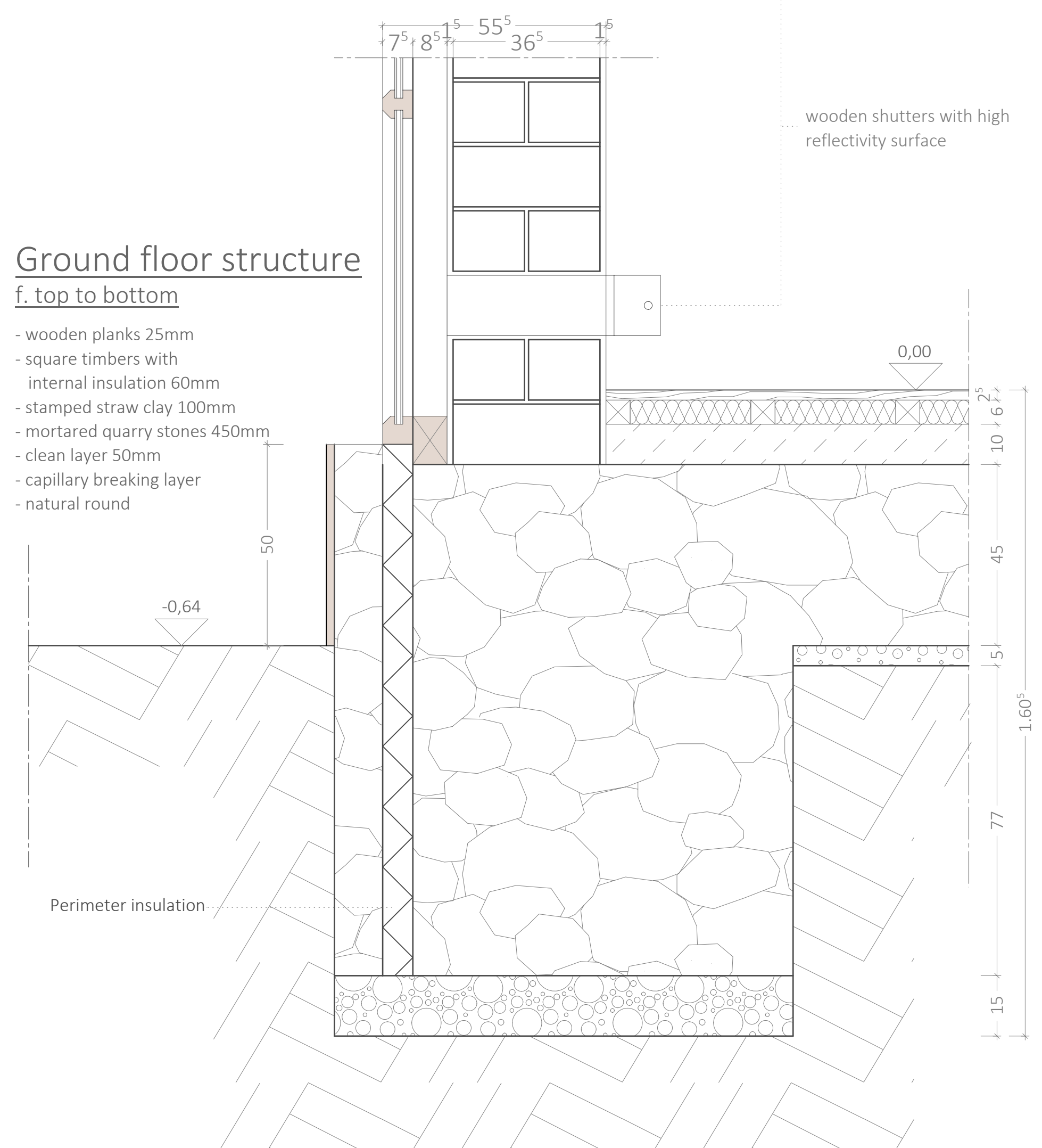
CONSTRUCTION DETAIL C M 1:10
