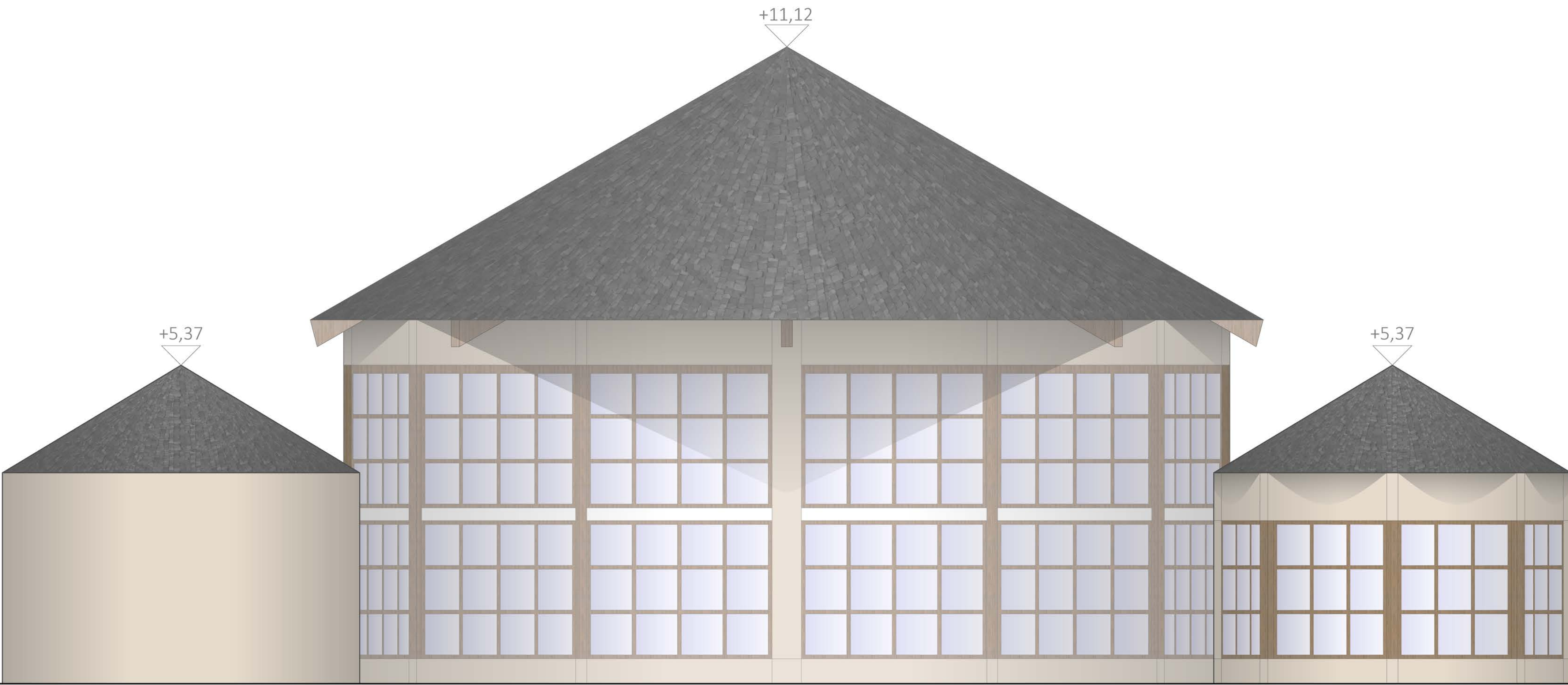
SOUTH ELEVATION M 1:50
